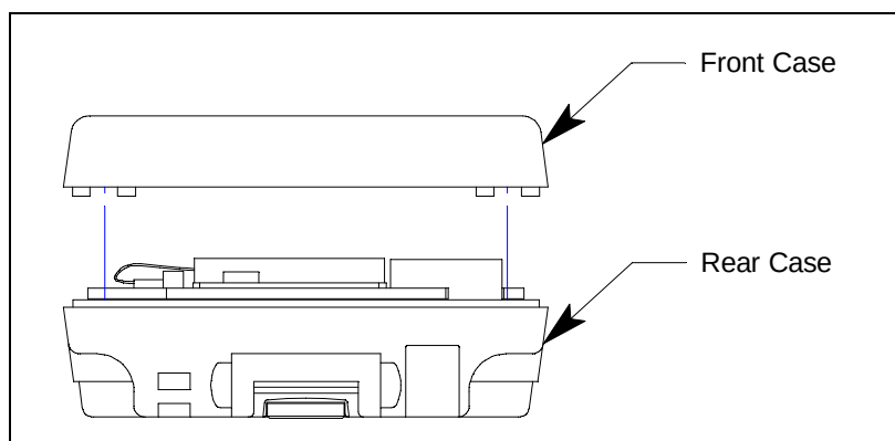
Figure 12: Case Separation
