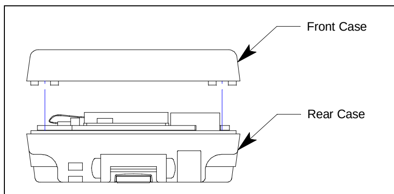
Figure 18: Case Separation
