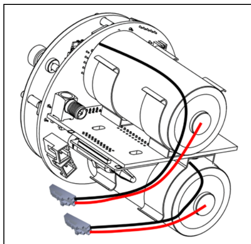
Figure 6: Battery Connection
