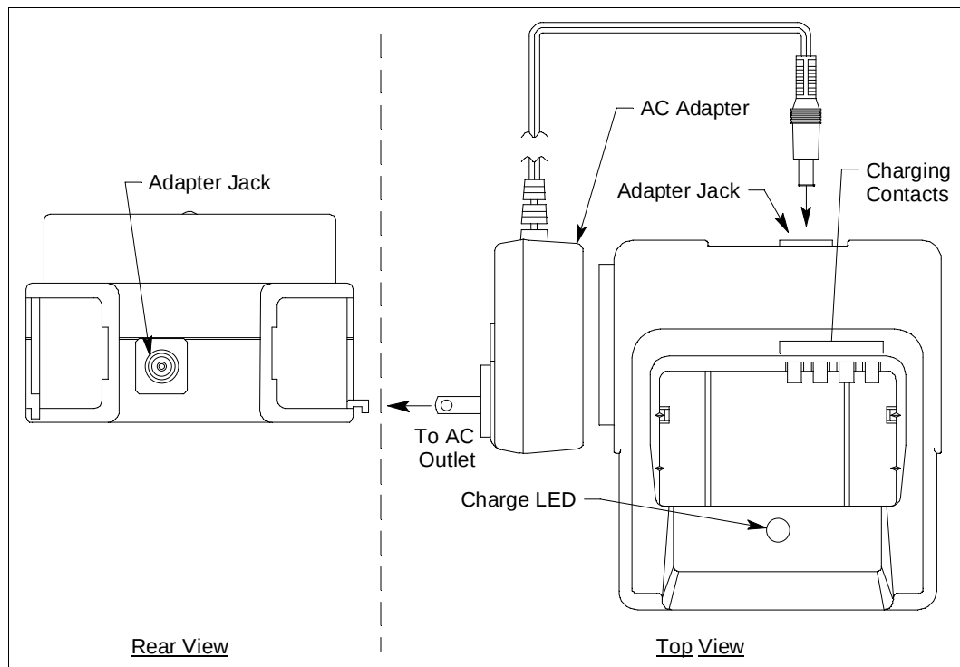
Figure 5: Gas Tracer AC Powered Charging Station
