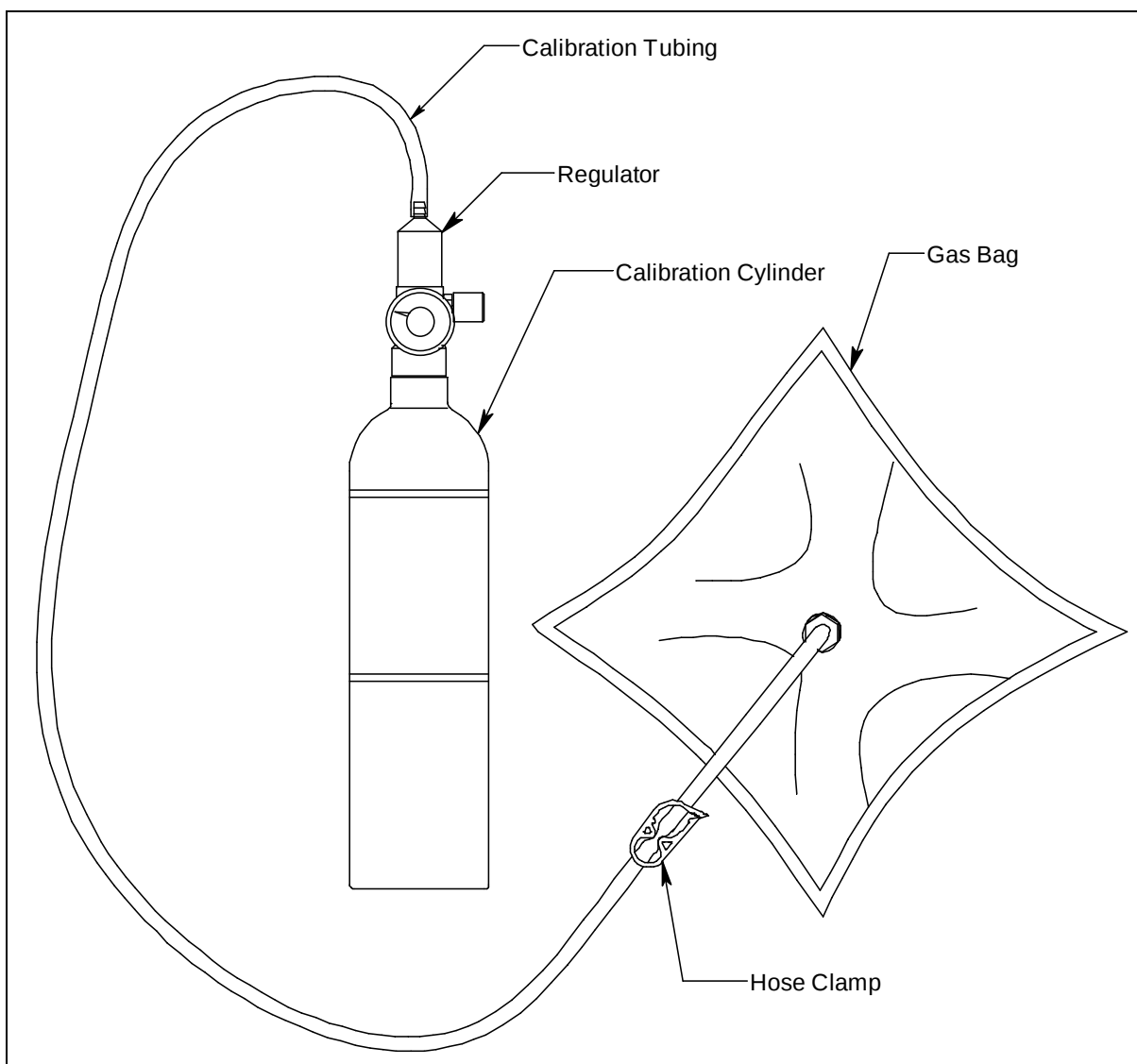
Figure 31: Gas Bag Calibration Kit
