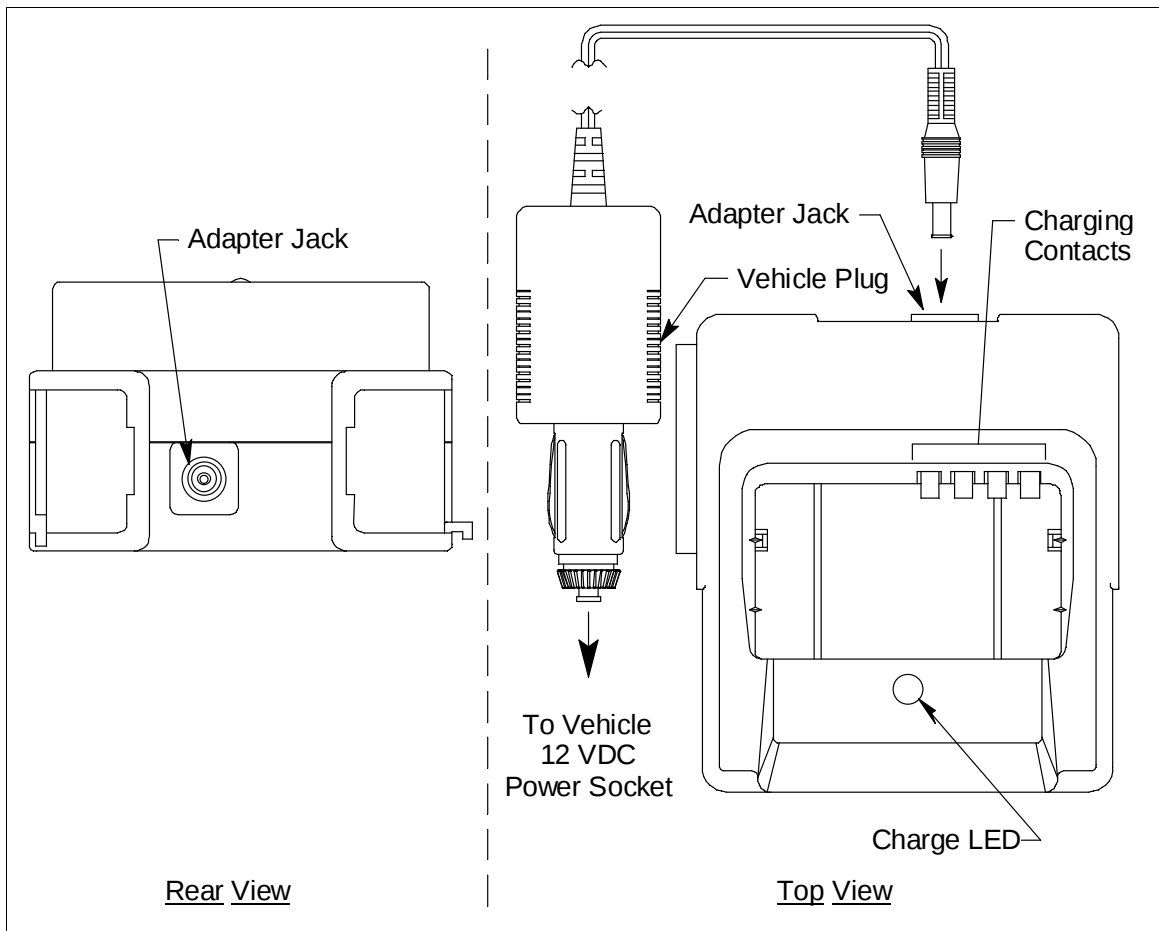
Figure 6: Gas Tracer DC Powered Charging Station
