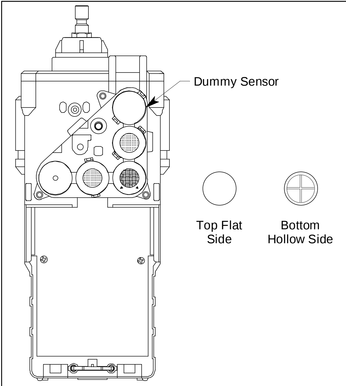
Figure 3: Dummy Sensors
