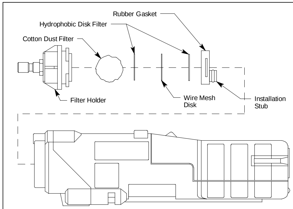
Figure 30: Changing the Filters & Wire Mesh Disk
