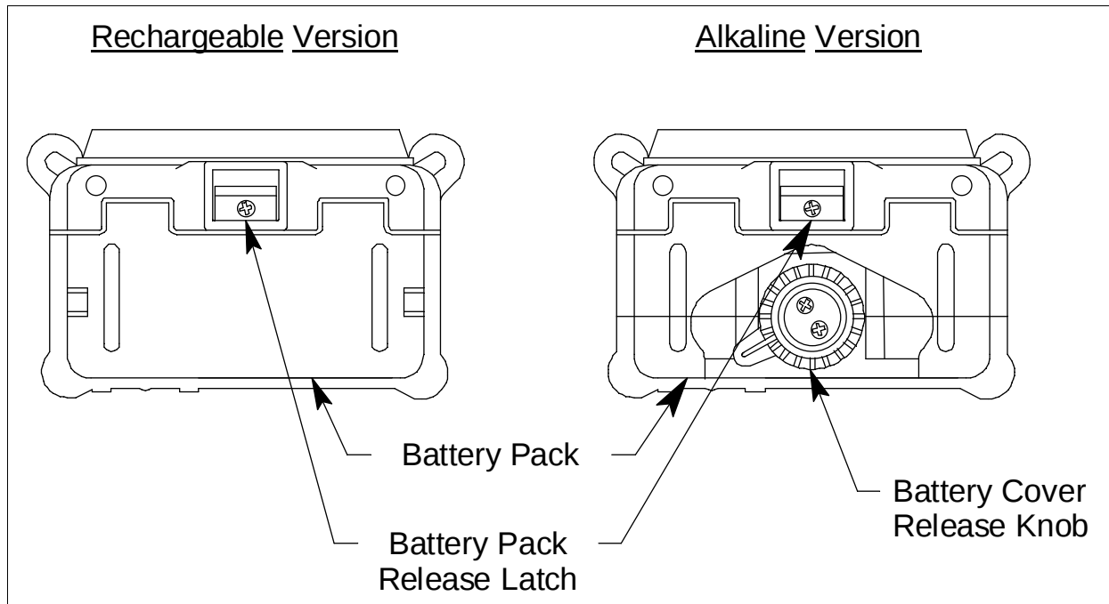
Figure 2: Components of the Gas Tracer, Bottom
